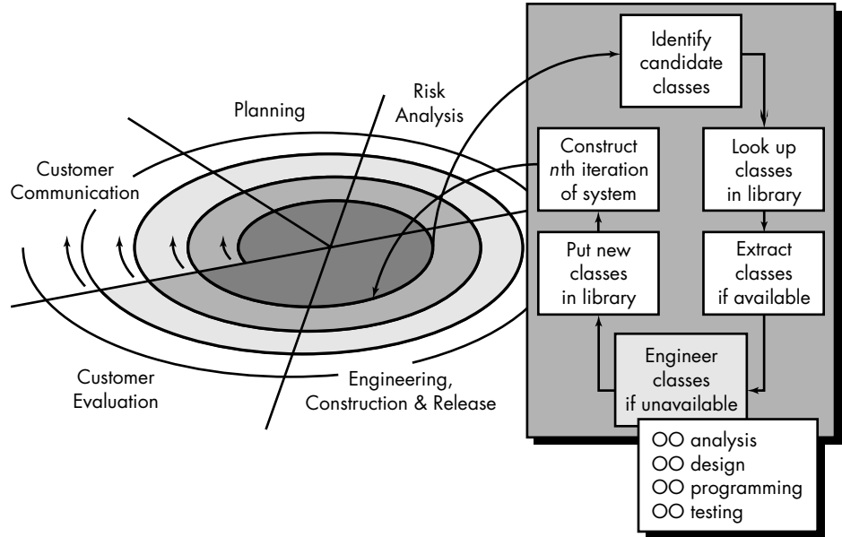
FIGURE 20.1 The OO process model
